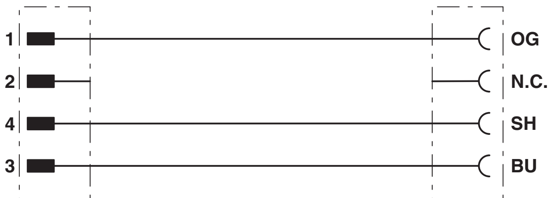
Circuit diagram
