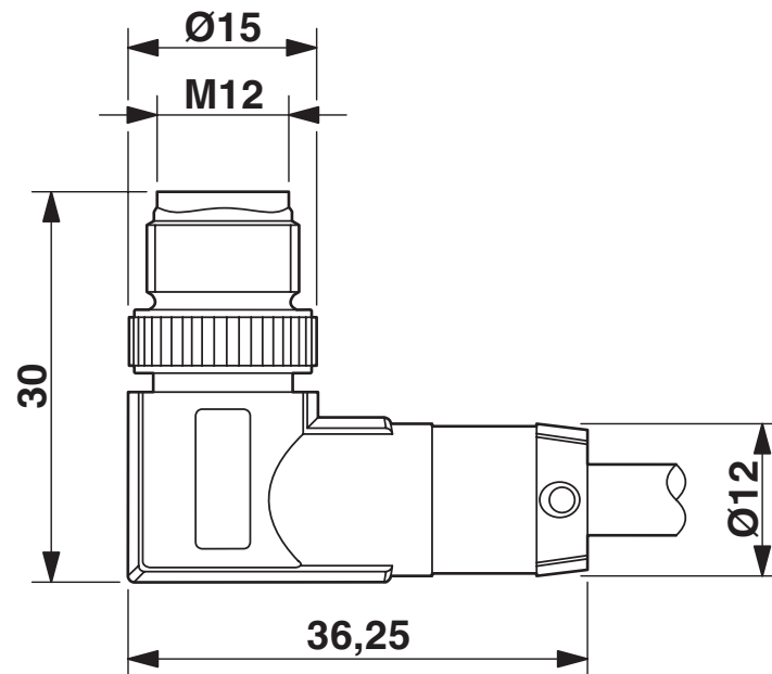
Dimensional drawing
