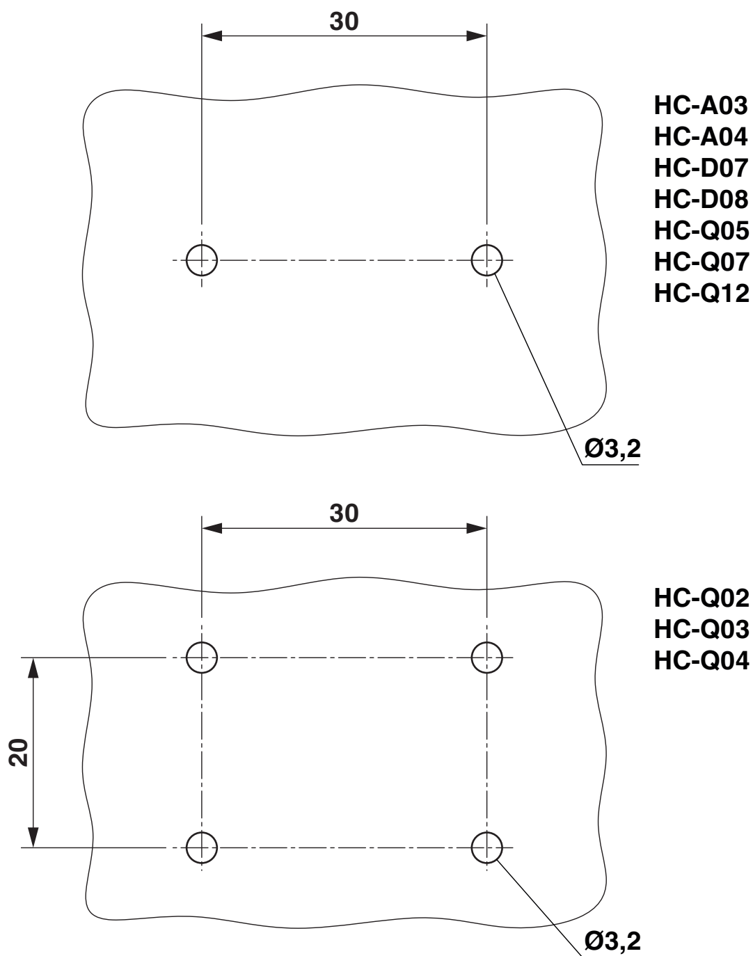
Dimensional drawing
