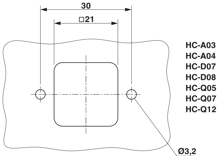
Dimensional drawing
