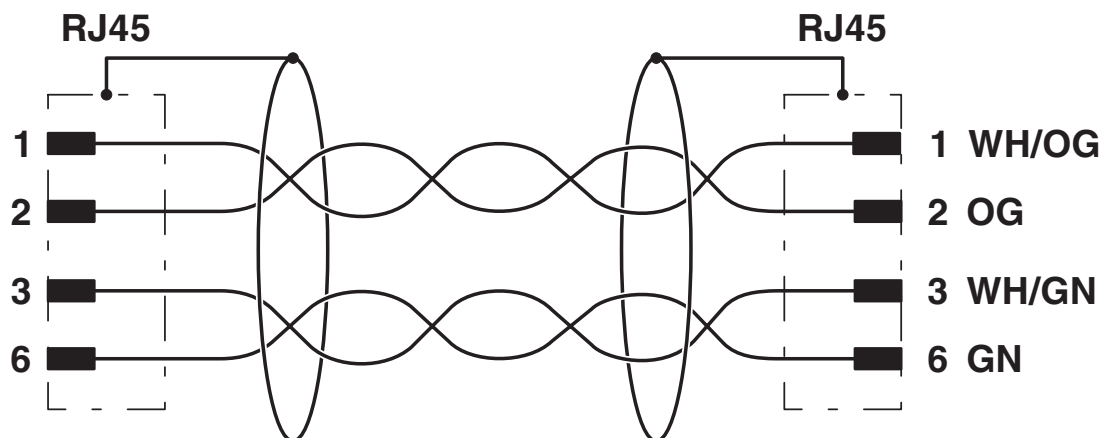
Circuit diagram
