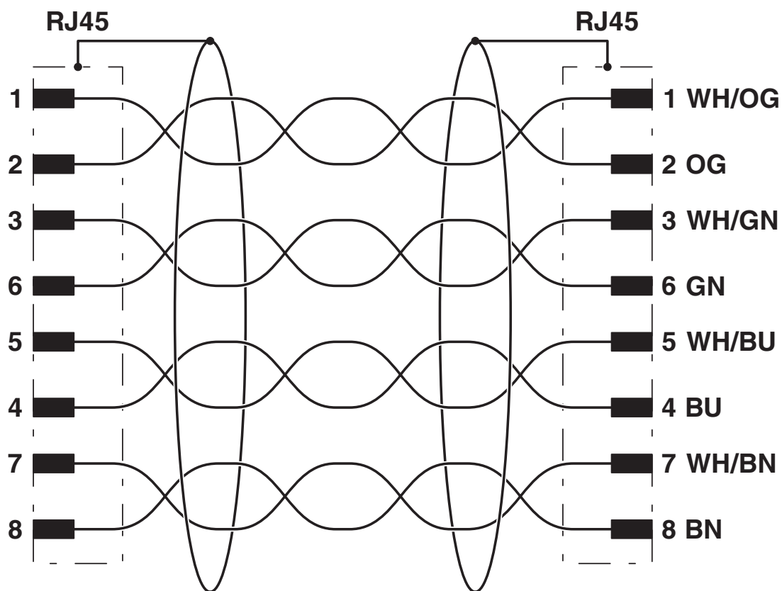
Circuit diagram
