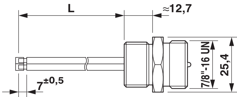
Dimensional drawing
