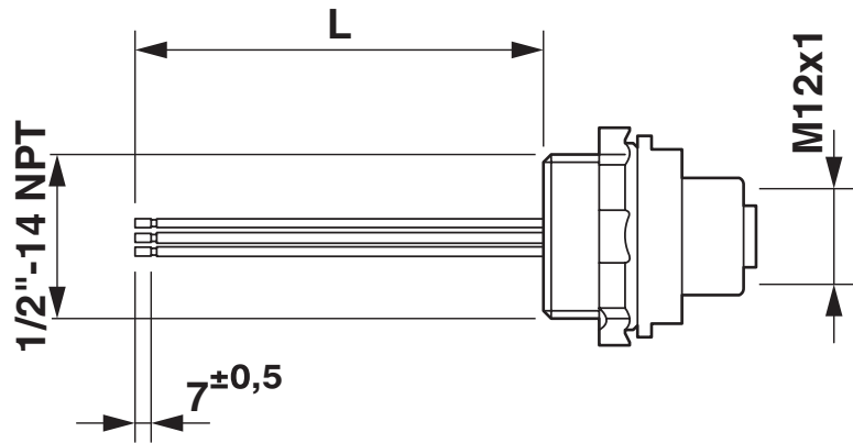
Dimensional drawing
