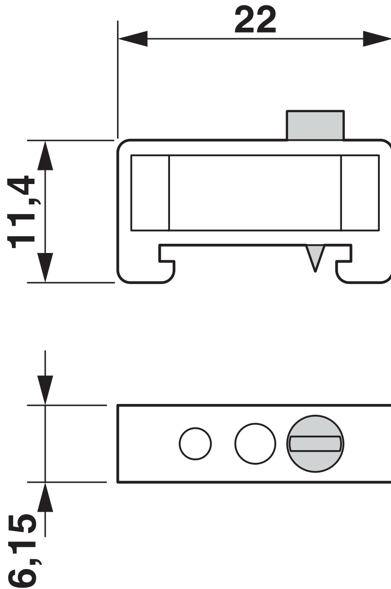
Dimensional drawing
