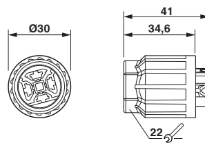
Dimensional drawing
