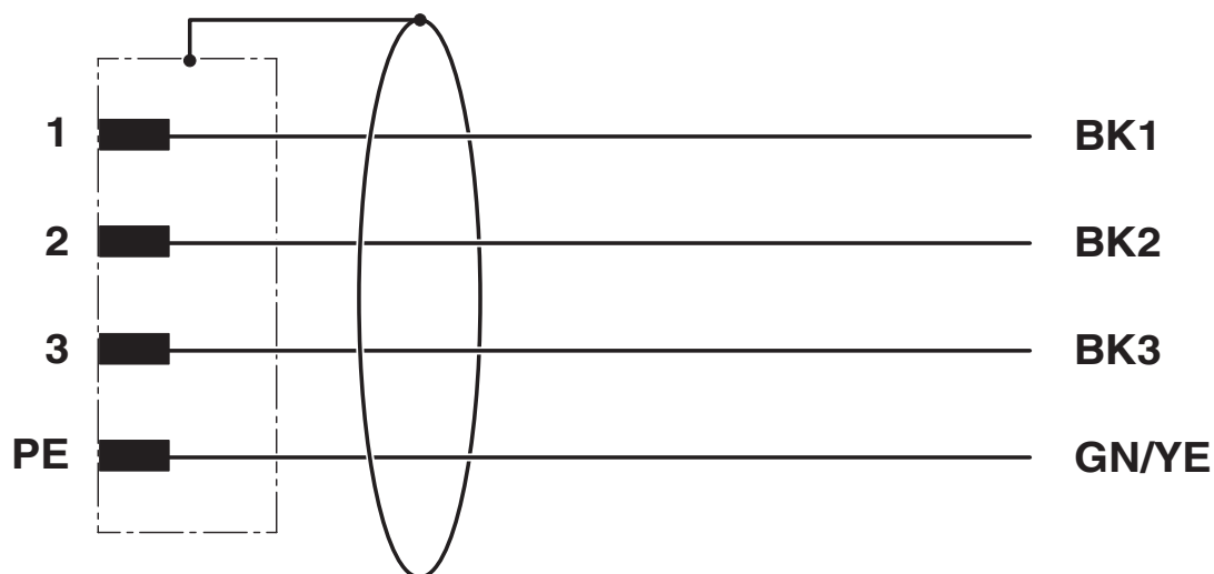
Circuit diagram
