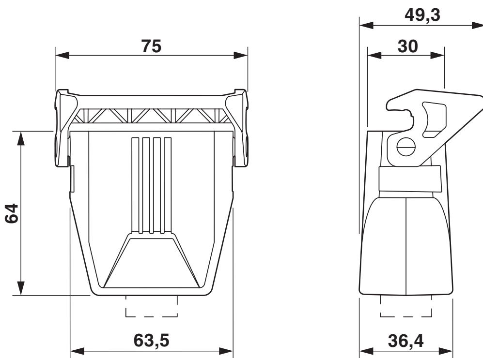
Dimensional drawing
