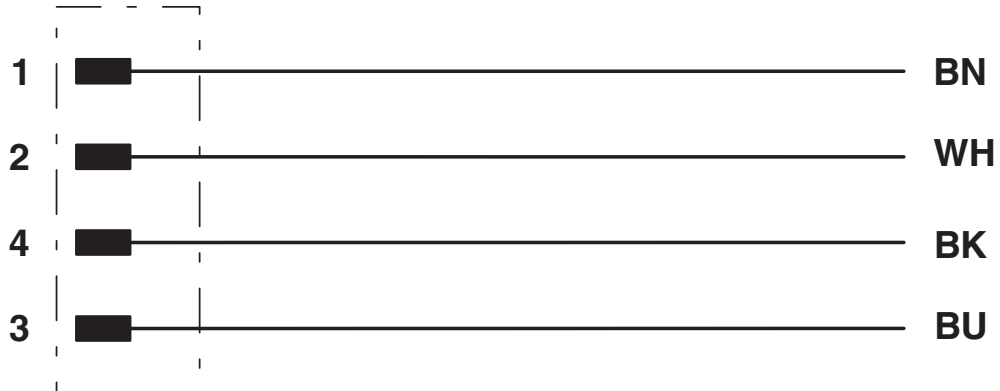
Circuit diagram
