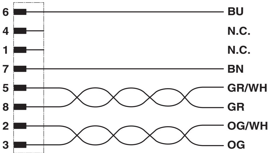
Circuit diagram
