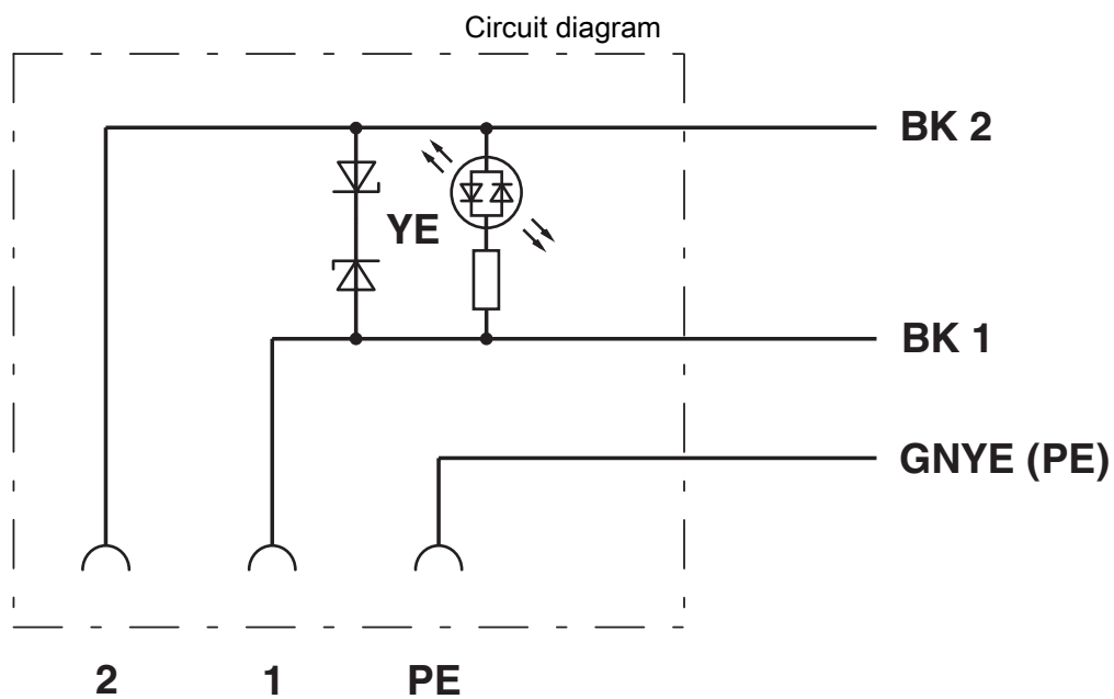
Valve connector, type BI, side view
