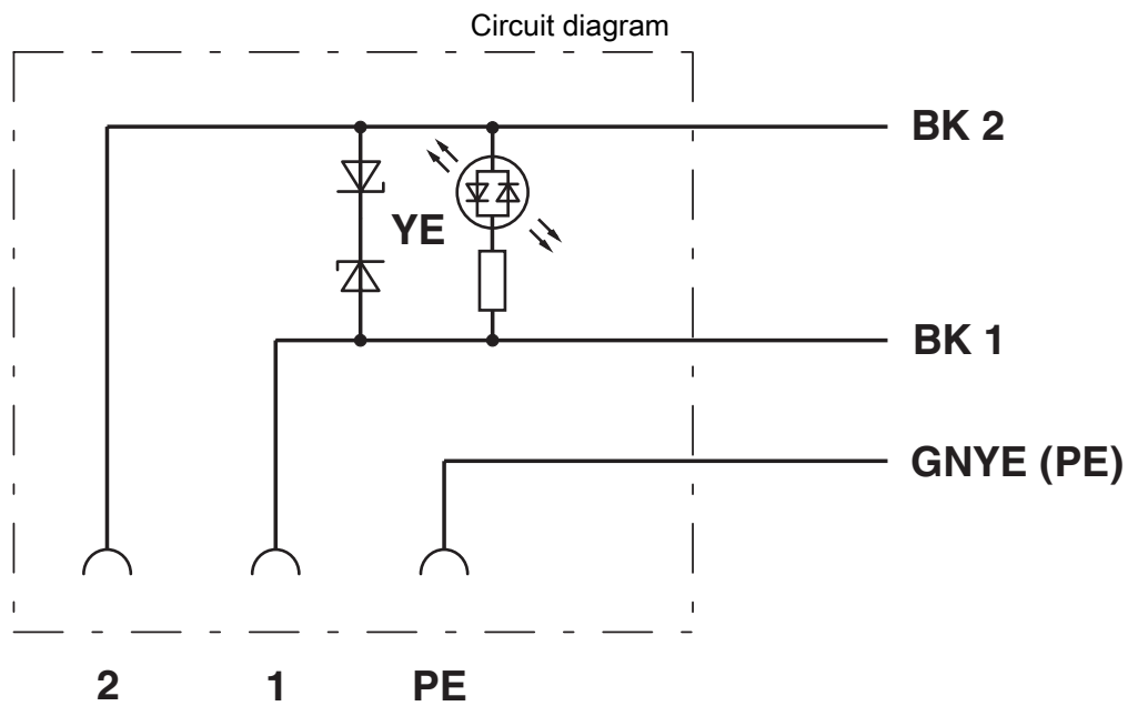
Valve connector, type B, side view
