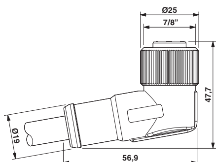
Dimensional drawing
