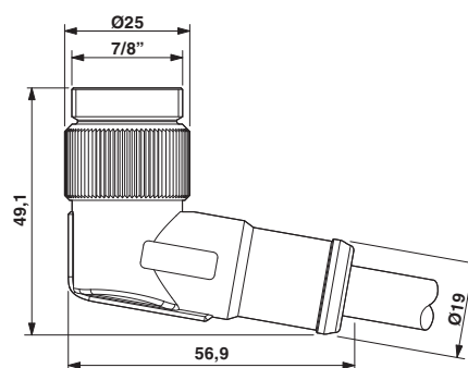
Dimensional drawing
