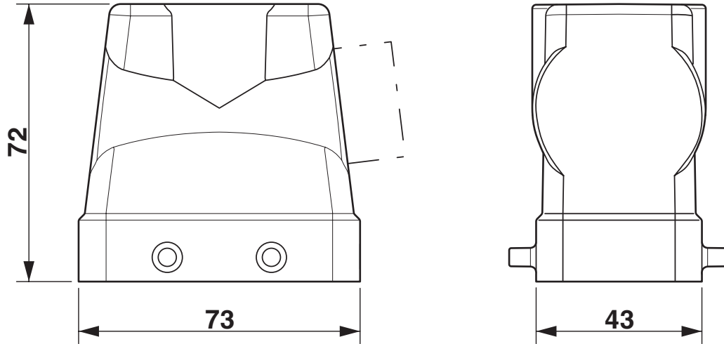
Dimensional drawing
