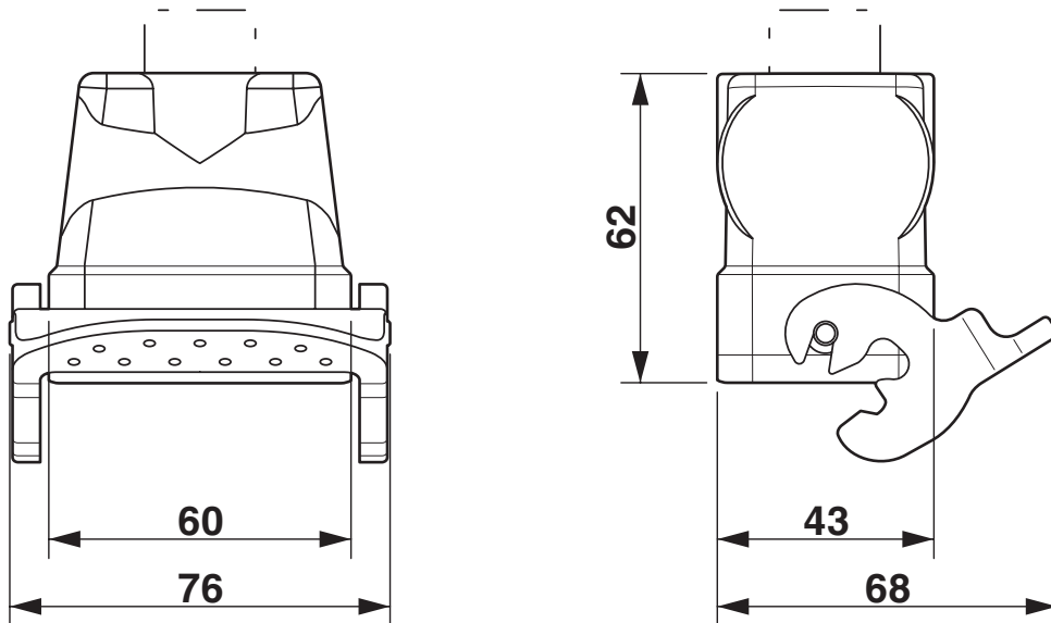
Dimensional drawing
