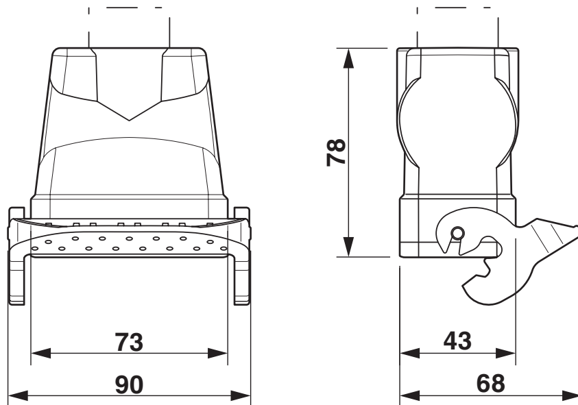
Dimensional drawing
