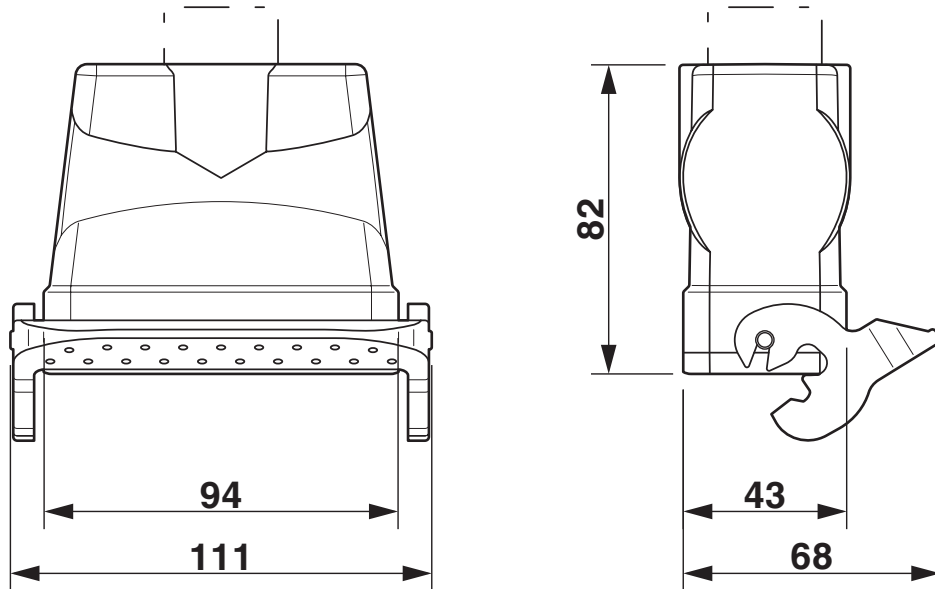
Dimensional drawing
