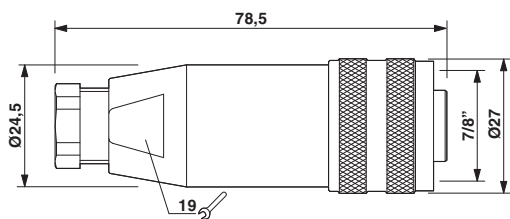
Dimensional drawing
