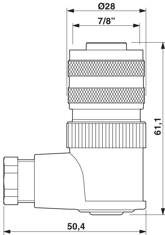
Dimensional drawing
