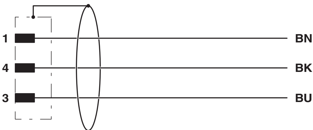
Circuit diagram
