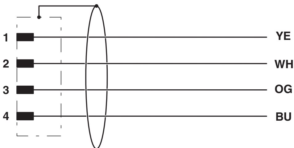
Circuit diagram
