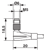
Dimensional drawing
