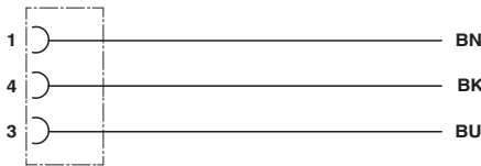
Contact assignment of the M5 socket
