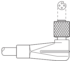
Layout of connector pin assignments
