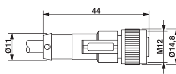
Dimensional drawing
