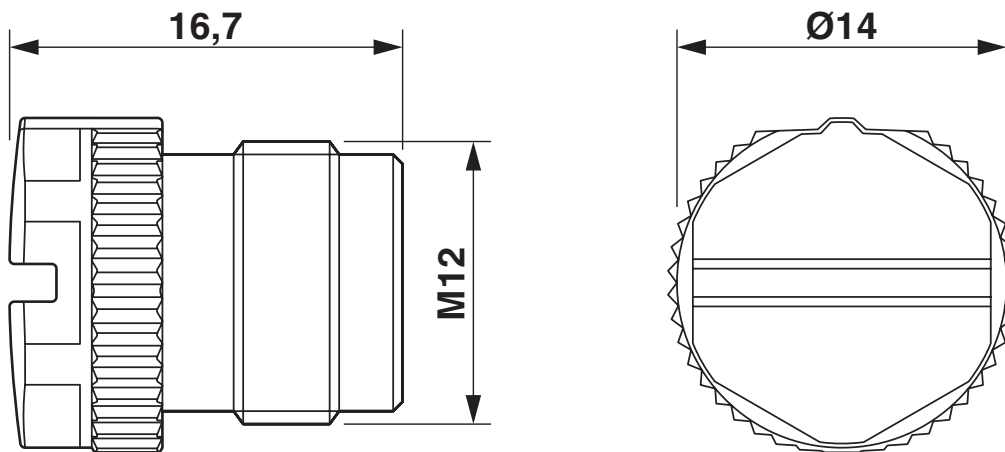
Dimensional drawing
