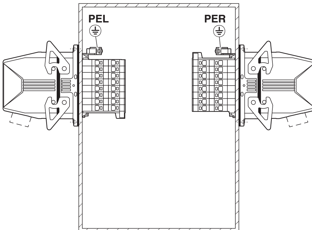
Mounting position PE connection left/right (PEL/PER)
