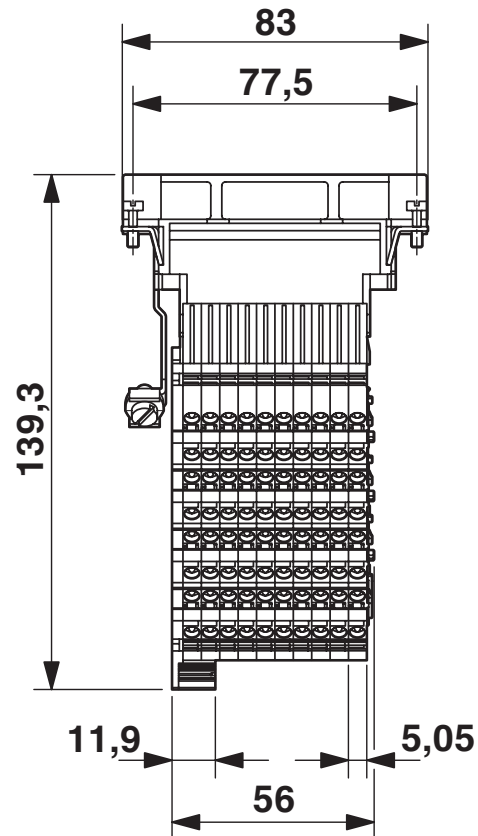
Dimensional drawing
