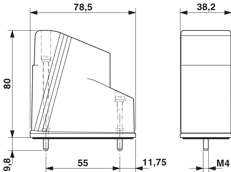
Dimensional drawing
