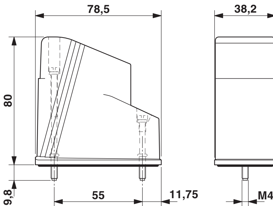
Dimensional drawing
