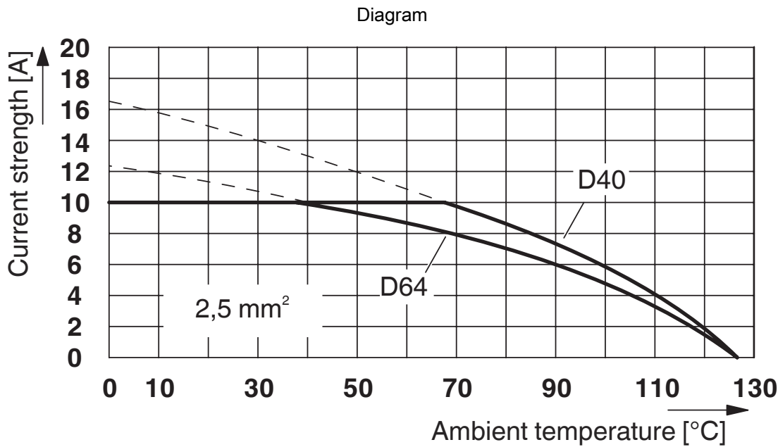
Derating diagram for 2,5 mm²
