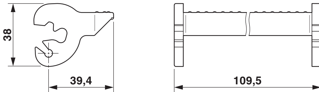
Dimensional drawing
