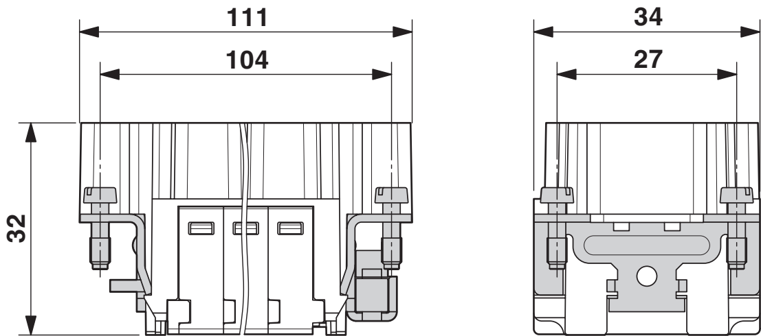
Dimensional drawing
