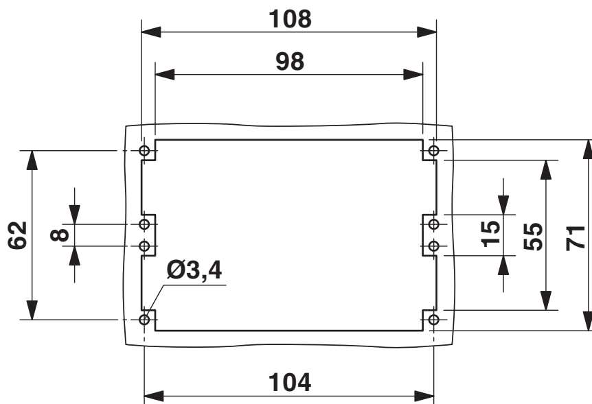
Mounting cutout when used without housing
