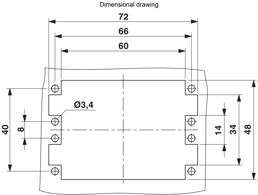
Mounting cutout when used without housing
