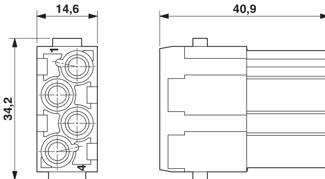
Dimensional drawing
