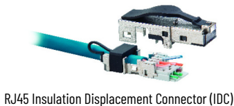
RJ45 Insulation Displacement Connector (IDC)
