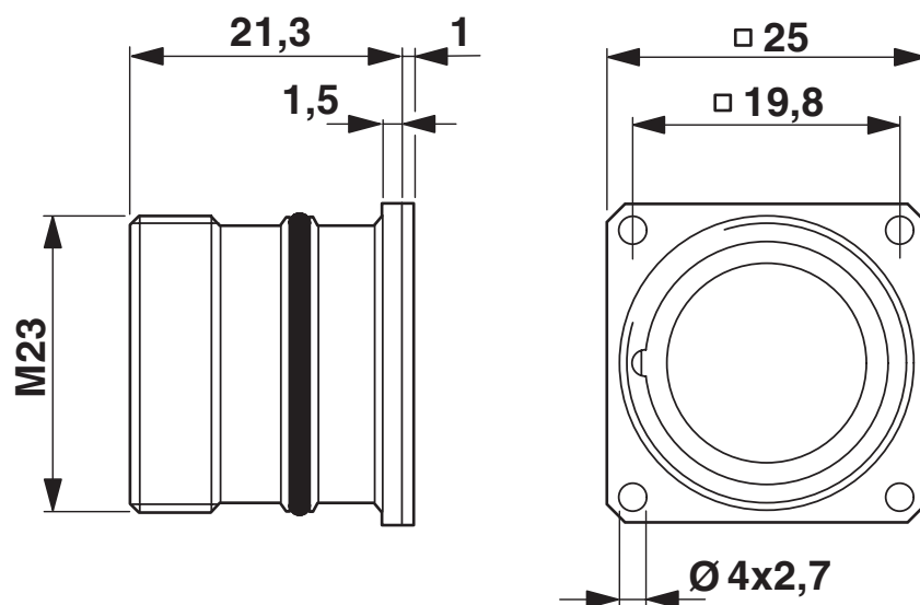
Dimensional drawing
