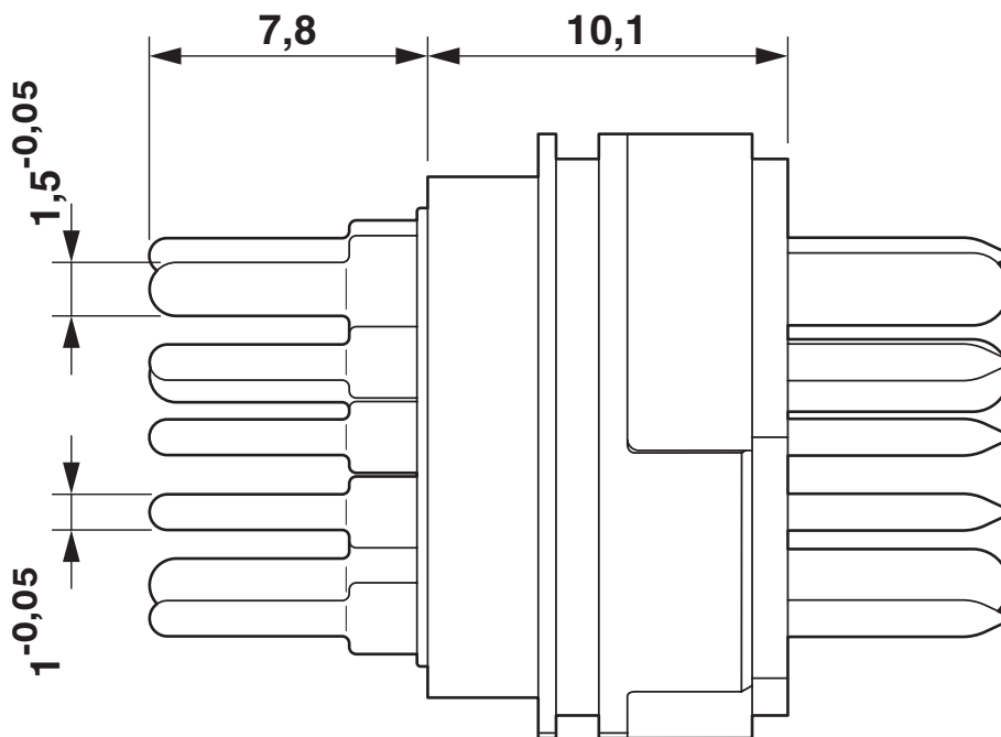
Dimensional drawing
