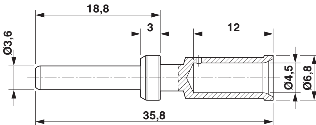
Dimensional drawing
