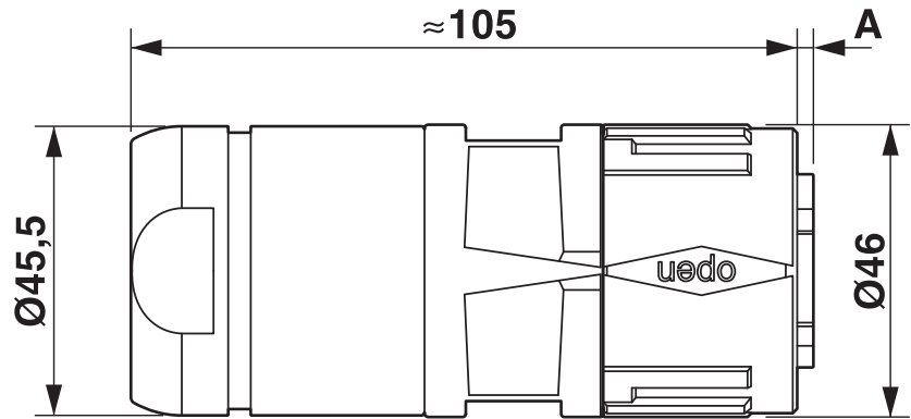
Dimensional drawing
