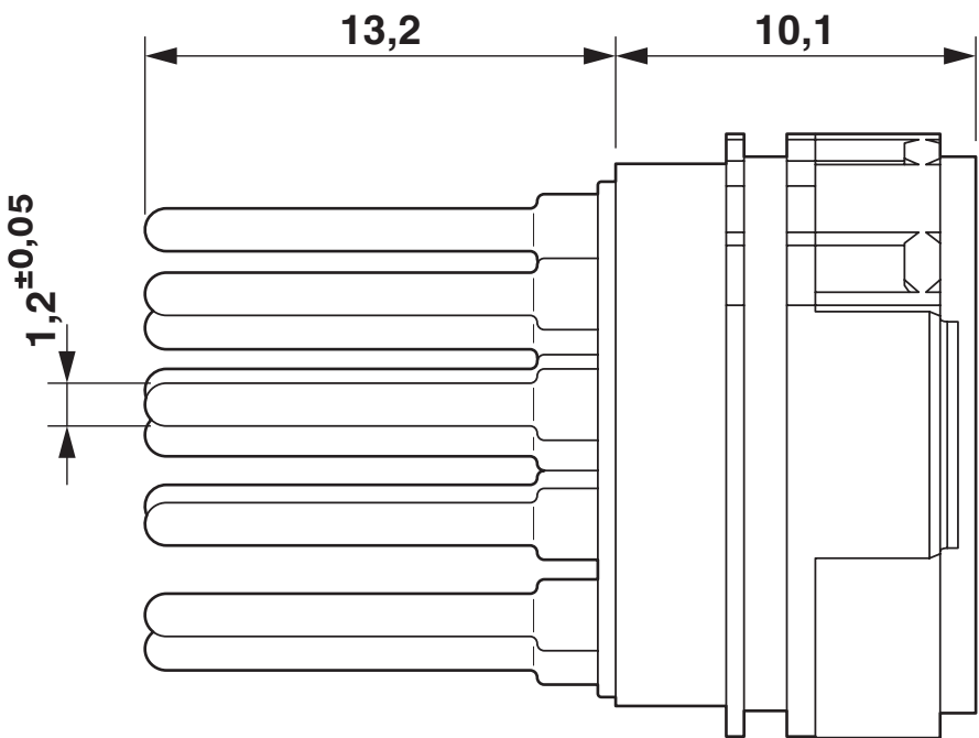
Dimensional drawing
