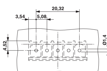
Drilling diagram
