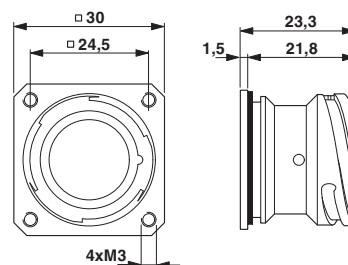
Dimensional drawing
