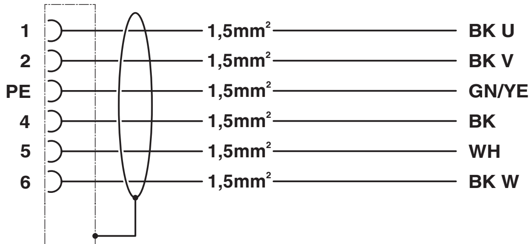
Circuit diagram
