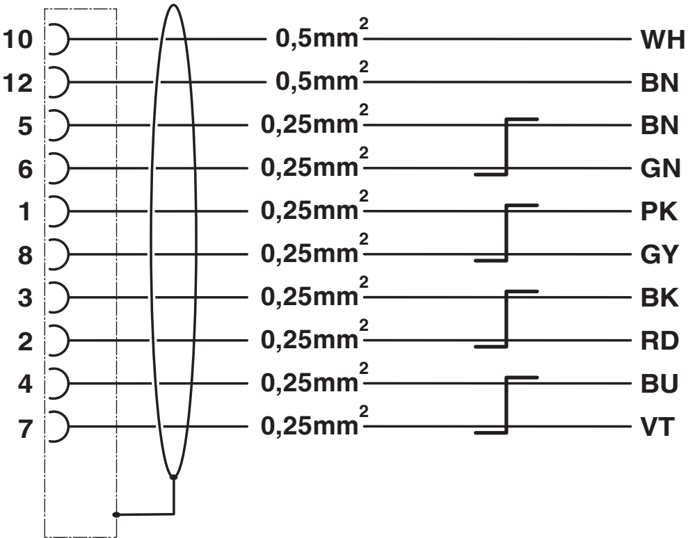
Circuit diagram
