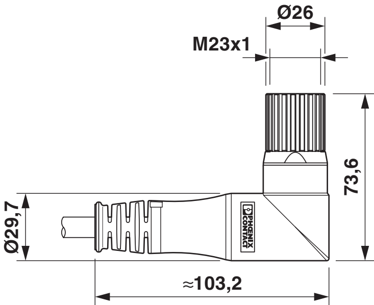
Dimensional drawing
